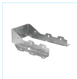
Face Mount Joist Hanger 托梁吊架
